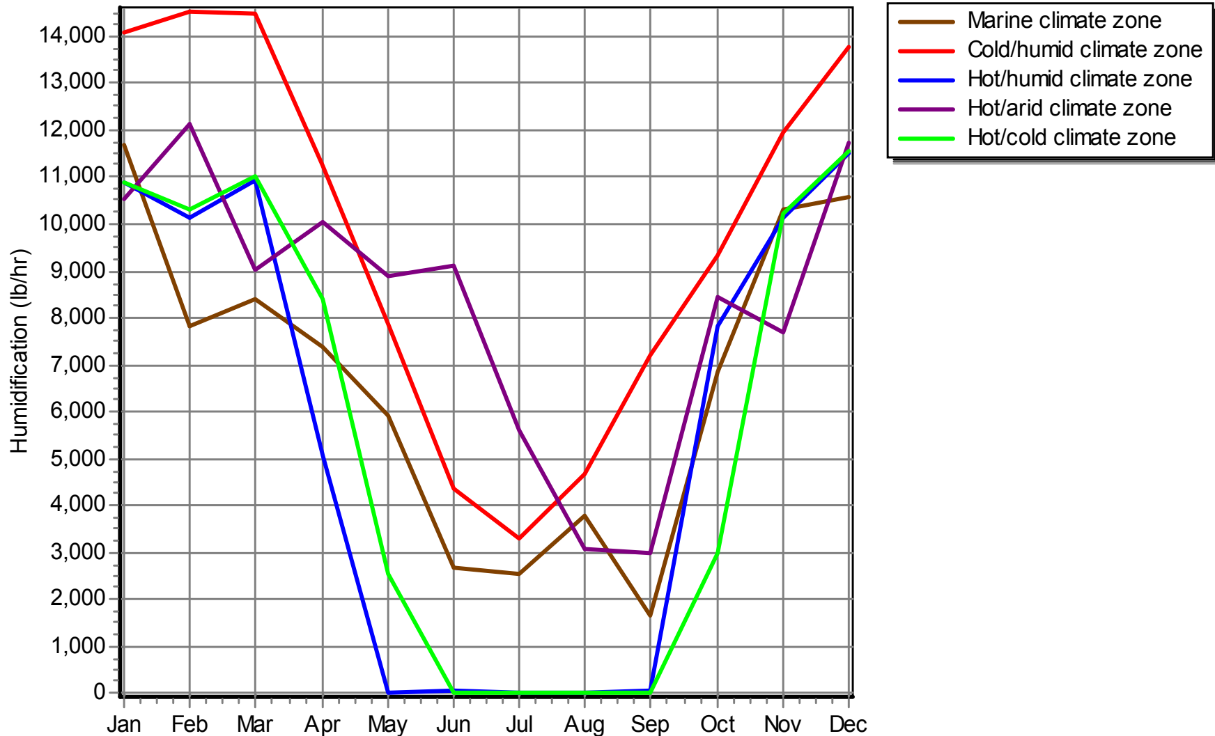
Peak Humidification Demand vs. Month By Simulation
