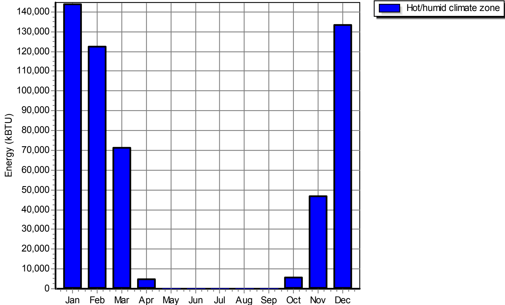
Total Annual HVAC Fuel Energy vs. Month By Simulation
