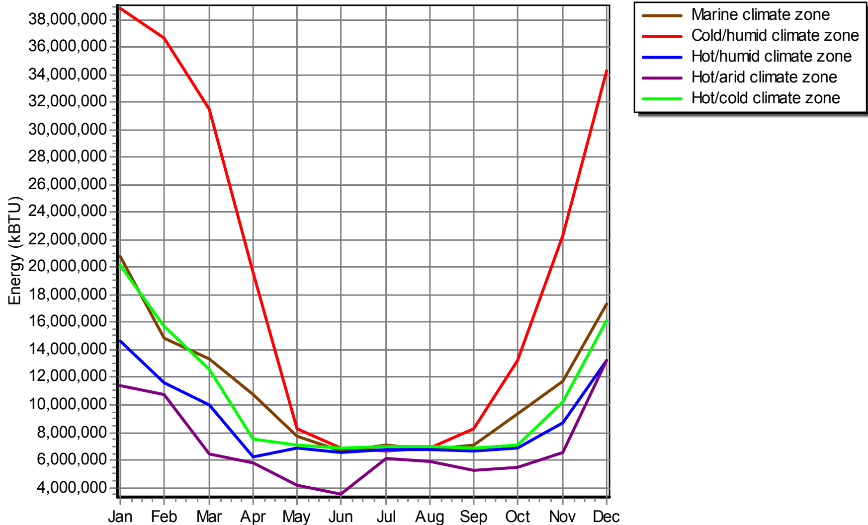
Total Makeup Air Heat Fuel Energy (External) vs. Month By Simulation
