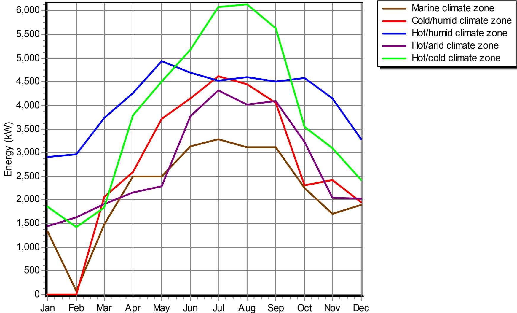
Peak Chiller Plant Energy Demand vs. Month By Simulation
