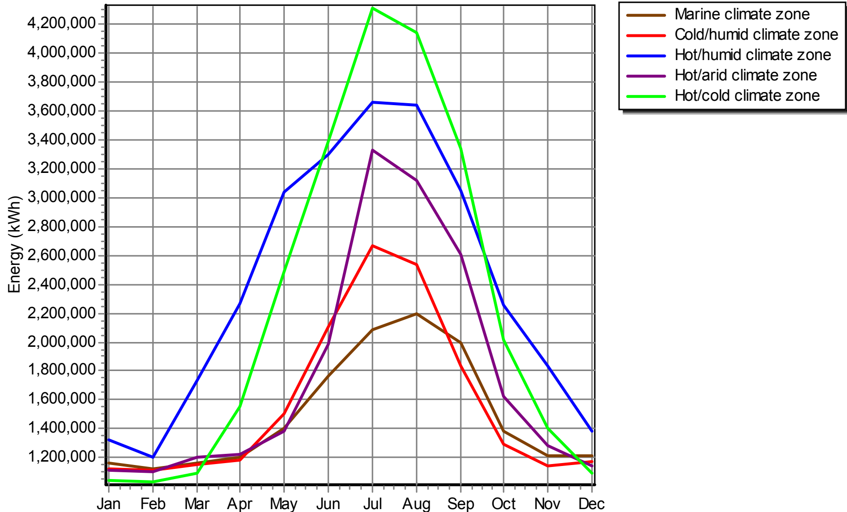
Total Annual HVAC Electric Energy vs. Month By Simulation
