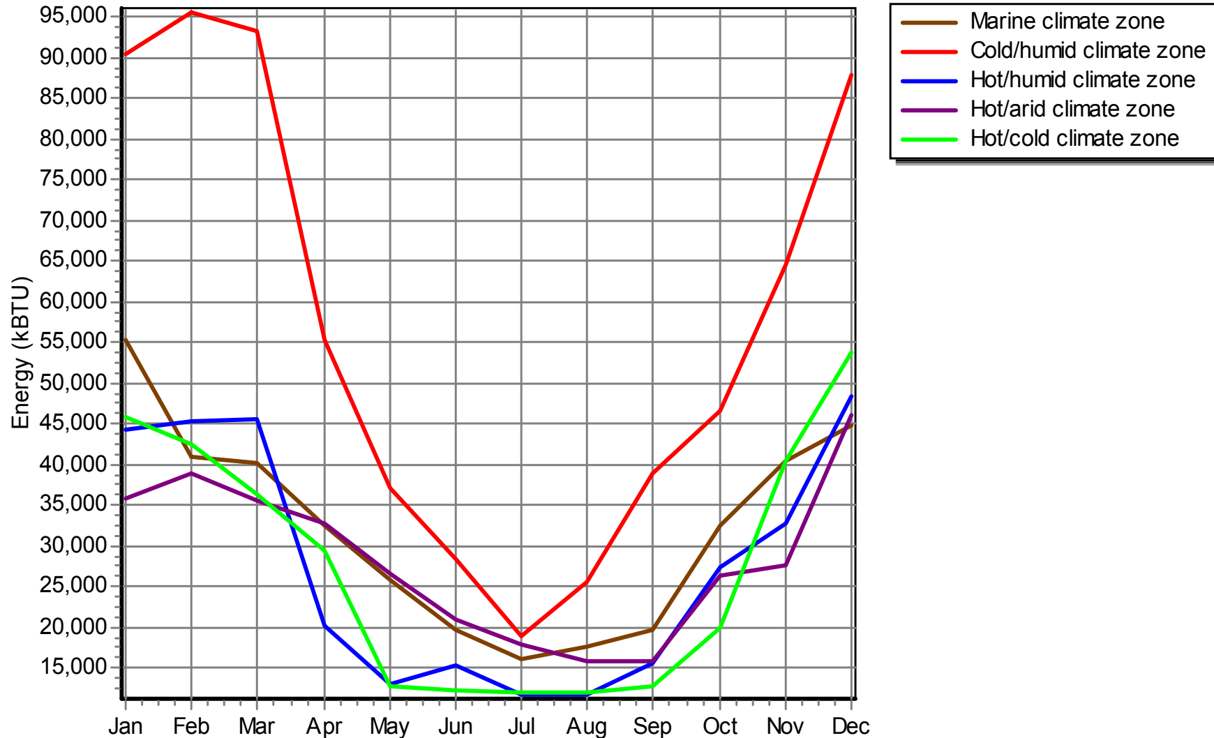
Peak Total Fuel Energy Demand vs. Month By Simulation
