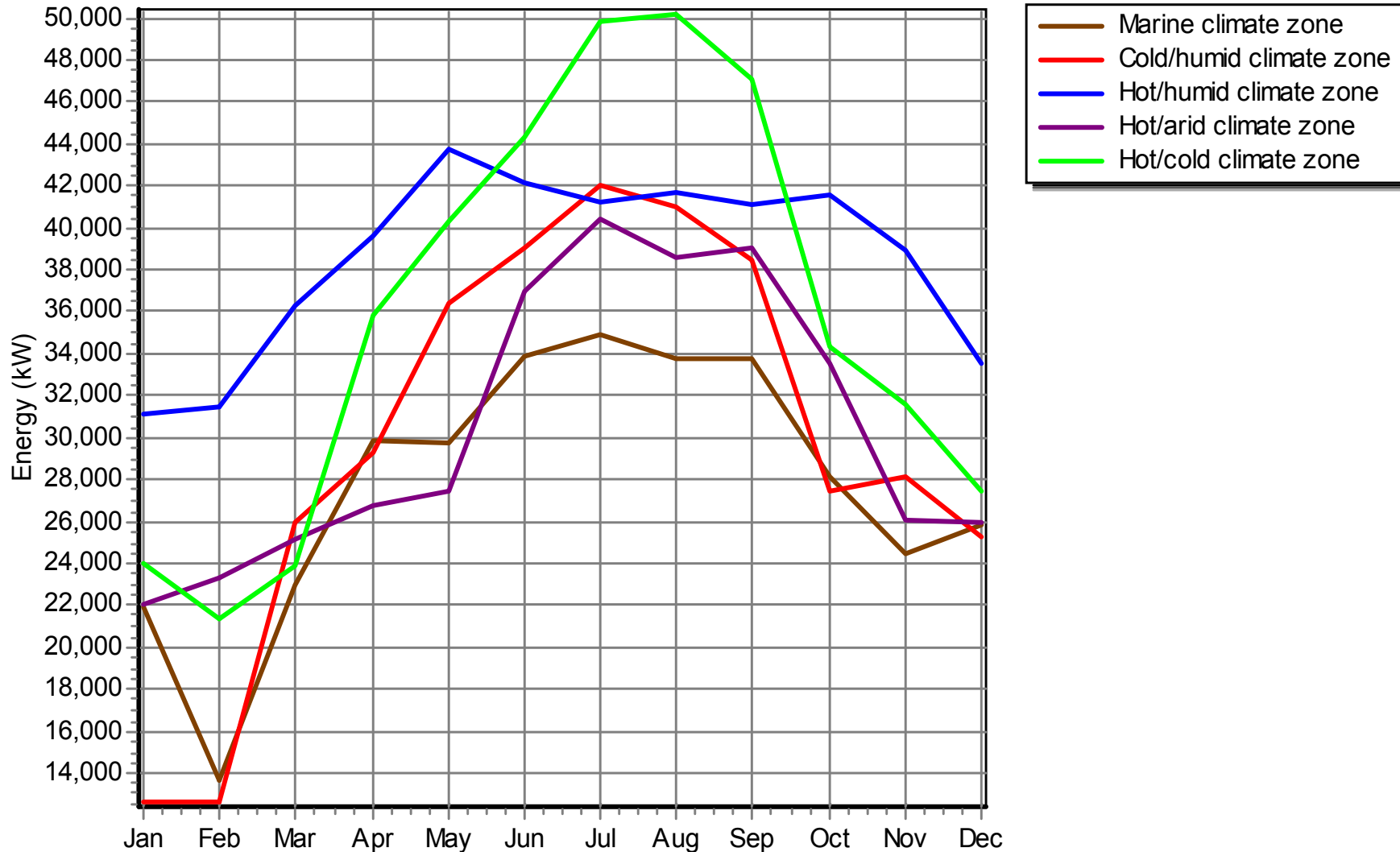
Peak Total Electric Energy Demand vs. Month By Simulation
