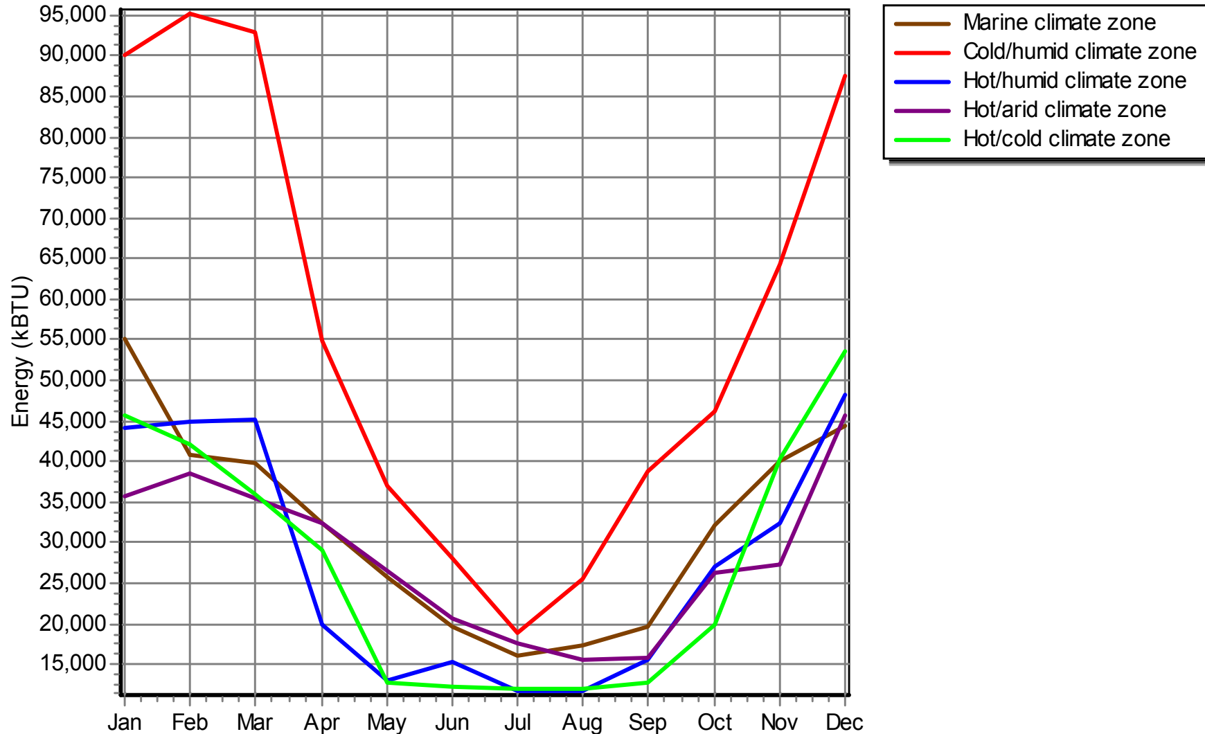
Peak Heating Fuel Energy Demand vs. Month By Simulation
